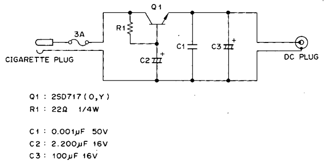
PG-3F CIRCUIT DIAGRAM
