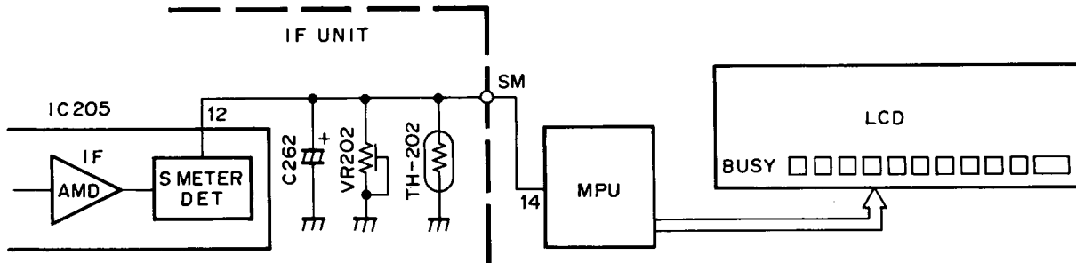
Fig. 4 S-Meter Circuit
