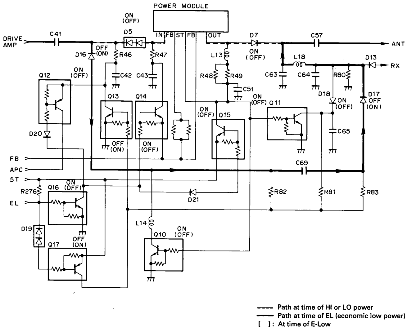
Fig.7 Economic Low-Power Circuit
