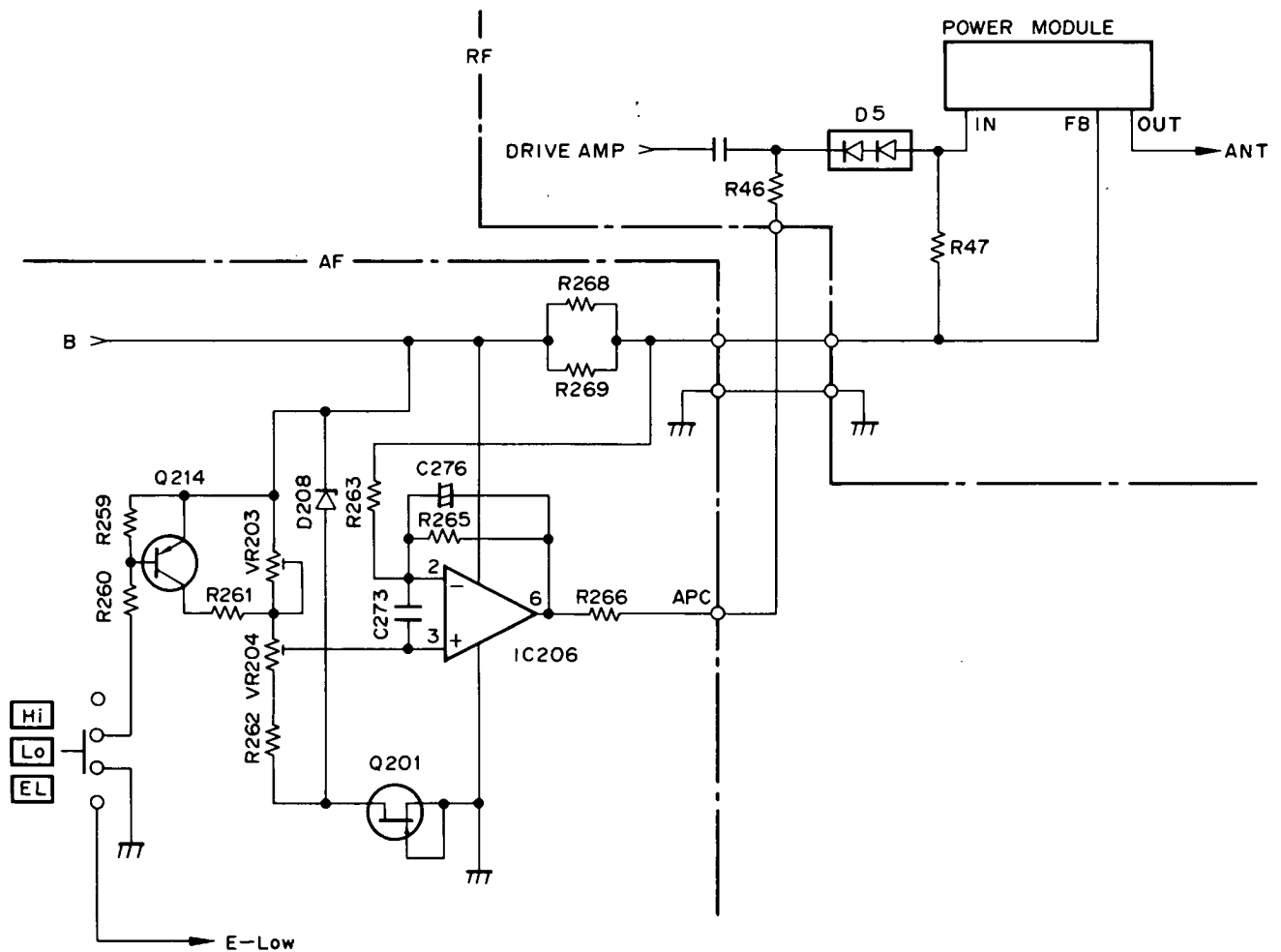
Fig. 6 APC Circuit and Transmitter output Switching Circuit
