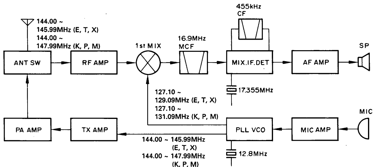
Fig. 1 Frequency configuration
